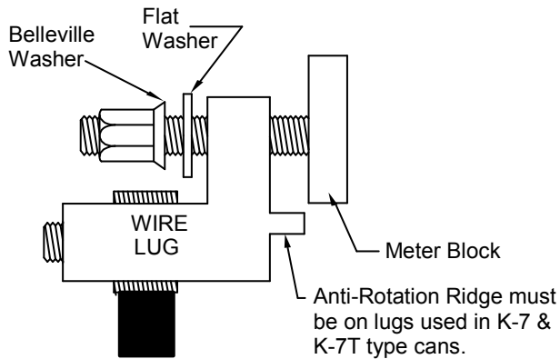
FIGURE IV-9 Lug-Type Meter Socket Installations
