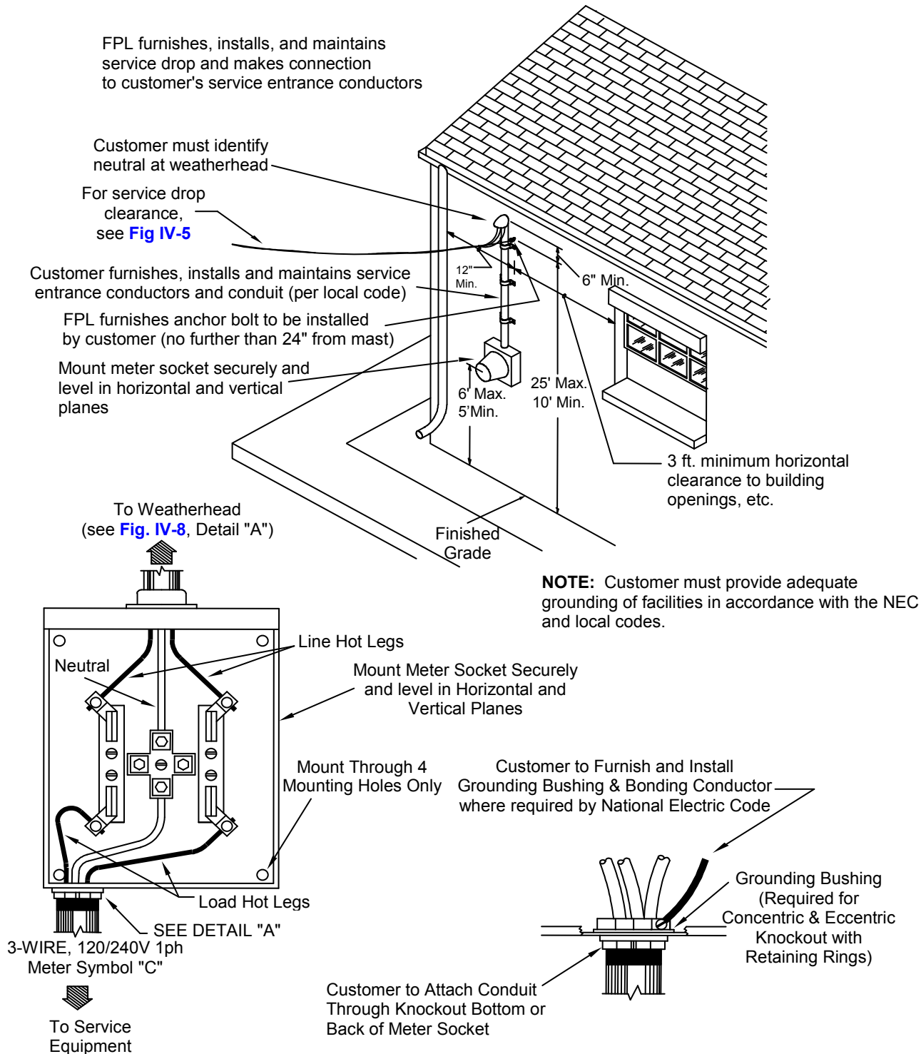
DETAIL "A"
