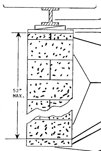
BLOCKING (Double Tiered and Blocks Interlocked)
